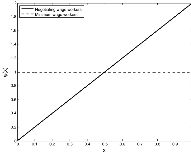
Figure 8: Comparing the \check{\psi}(x) and \bar{\psi}(x) densities, example with \beta = 1/2 and \chi = 1
