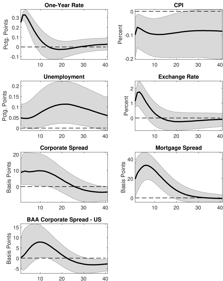
Figure 5 IRFs TO A MONETARY POLICY SHOCK - 2 INSTRUMENTS. Note. VAR estimated in log levels, with 2 lags, and a constant over the period 1992:1-2015:1. The IRFs are computed using the first column of B matrix from equation (10). First stage results: F-Statistic: 12.3 and R^2 = 0.11 . The solid and dashed lines report the mean and the 68% confidence intervals computed using moving block bootstrap with 5,000 replications.
