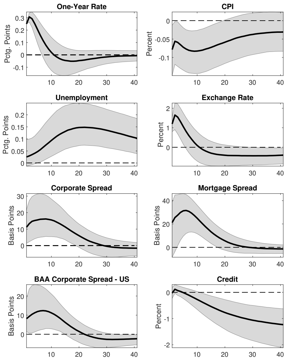
Figure B2 IRFs TO A MONETARY POLICY SHOCK - FULL SPECIFICATION. Note. VAR estimated in log levels, with 2 lags, and a constant over the 1992:1-2015:1 period. The 1-year Government Gilt Yield is instrumented using the second front contract of 3-month Sterling future. First stage results: F-Statistic: 23.8 and R^2 = 0.08 . The solid and dashed lines report the mean and the 68% confidence intervals computed using moving block bootstrap with 5,000 replications.
