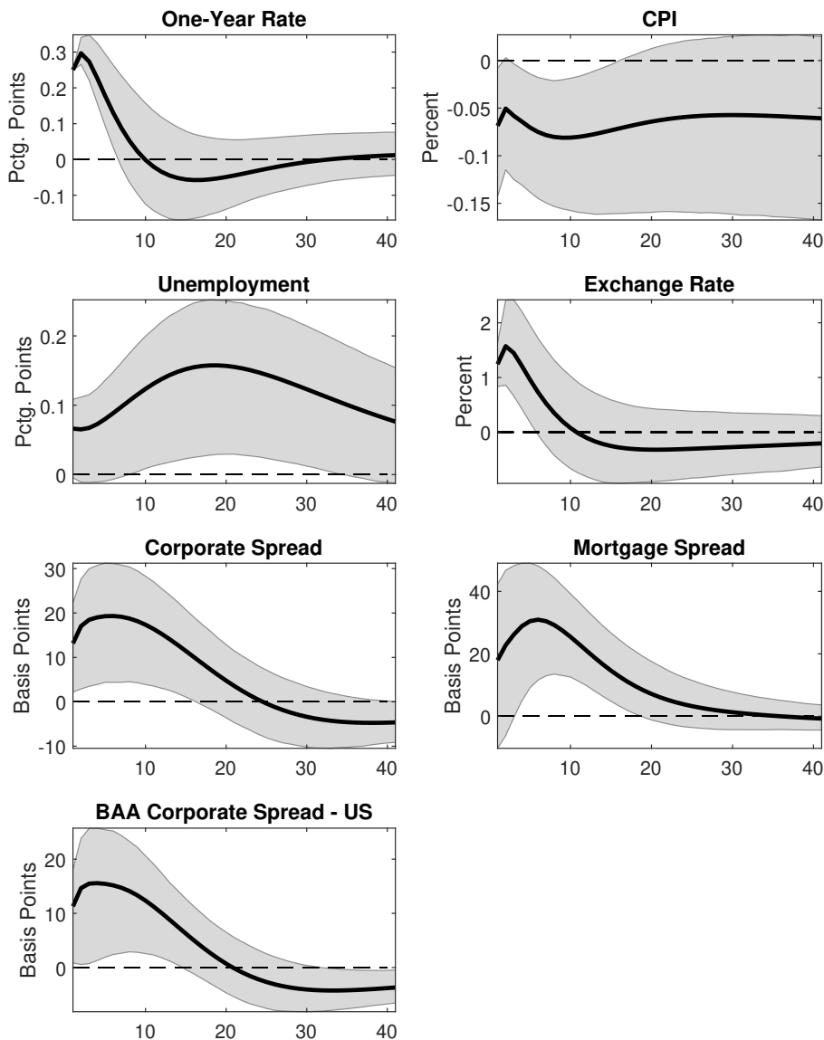
Figure 2 IRFs TO A MONETARY POLICY SHOCK - BASELINE SPECIFICATION. Note. VAR estimated in log levels, with 2 lags, and a constant over the period 1992:1-2015:1. The 1-year Government Gilt Yield is instrumented using the second front contract of 3-month Sterling future. First stage results: F-Statistic: 23.4 and R^2 = 0.08 . The solid and dashed lines report the mean and the 68% confidence intervals computed using moving block bootstrap with 5,000 replications.
