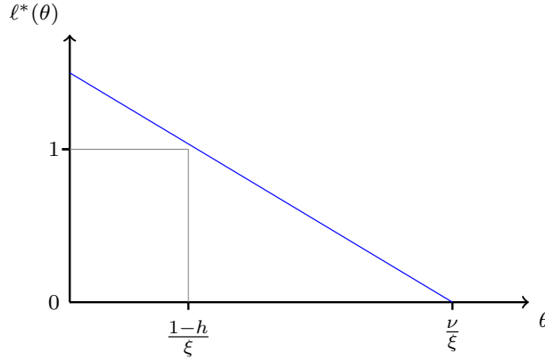
Figure 1.3: Threshold \ell^*(\theta) .
