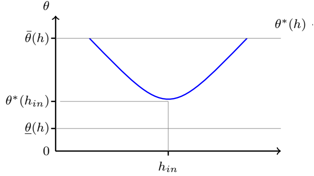
Figure 1.4: Threshold as a function of haircut.
