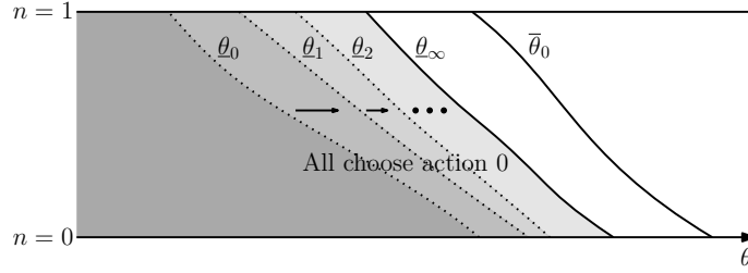
Figure 5: Convergence of iterations from the left
