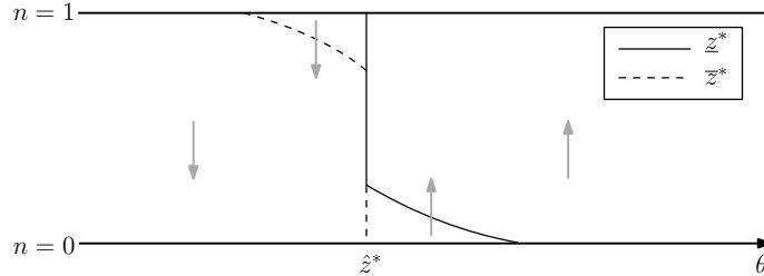
Figure 21: Equilibrium when \delta \rightarrow \infty
