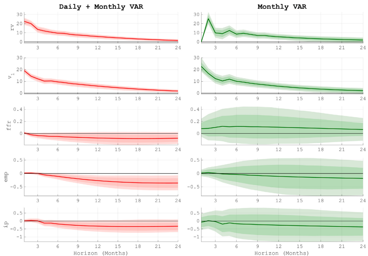
Fig. 3. Daily versus monthly identification in BDG.
