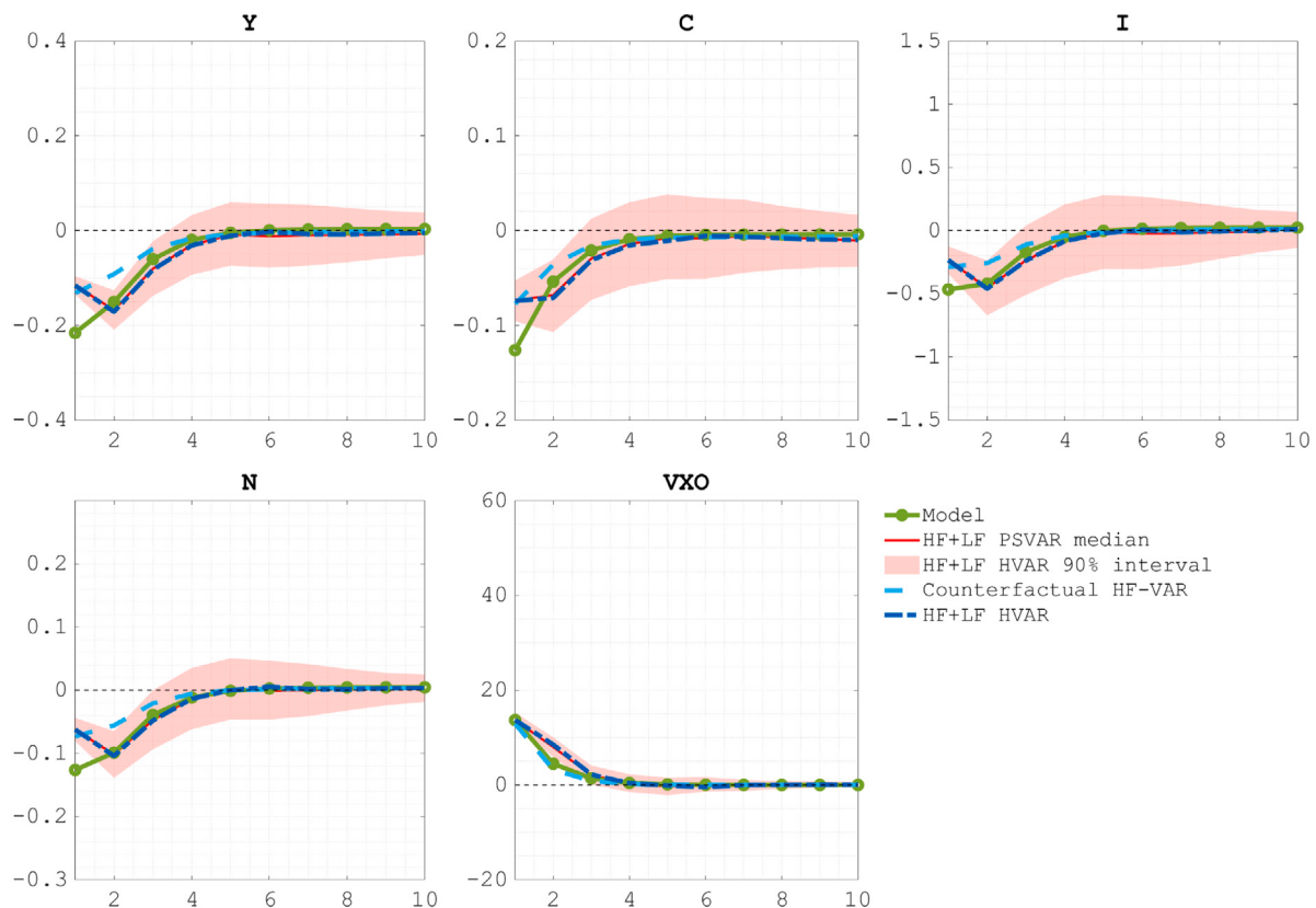
Fig. 1. True and estimated IRFs in the BB model.
