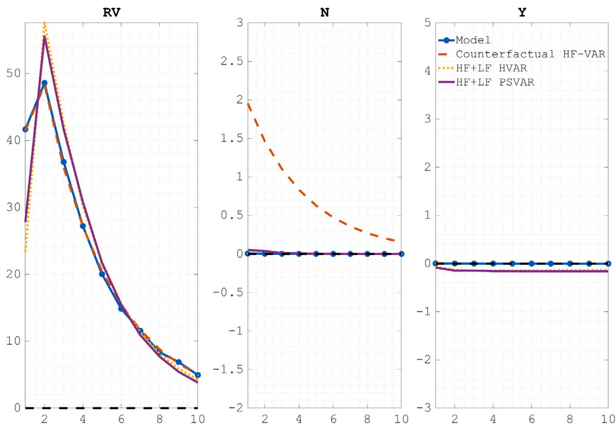
Fig. 2. True and estimated IRFs in the RSBC model.
