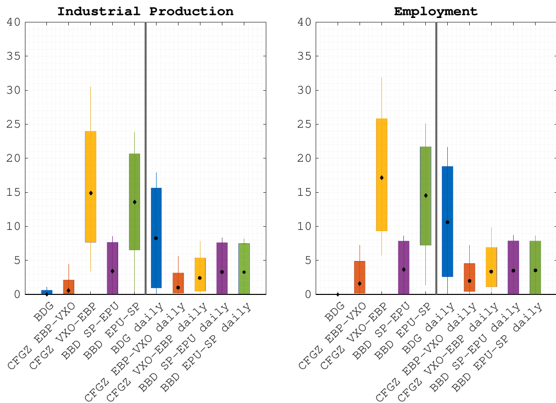
Fig. 7. FEV Contribution of Uncertainty Shocks across models and identification schemes.
