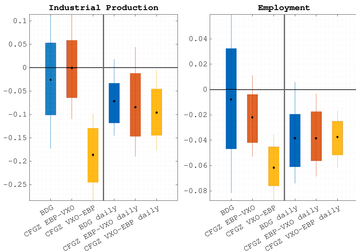
Fig. 6. Cumulative impact of uncertainty shocks across models and identification schemes.
