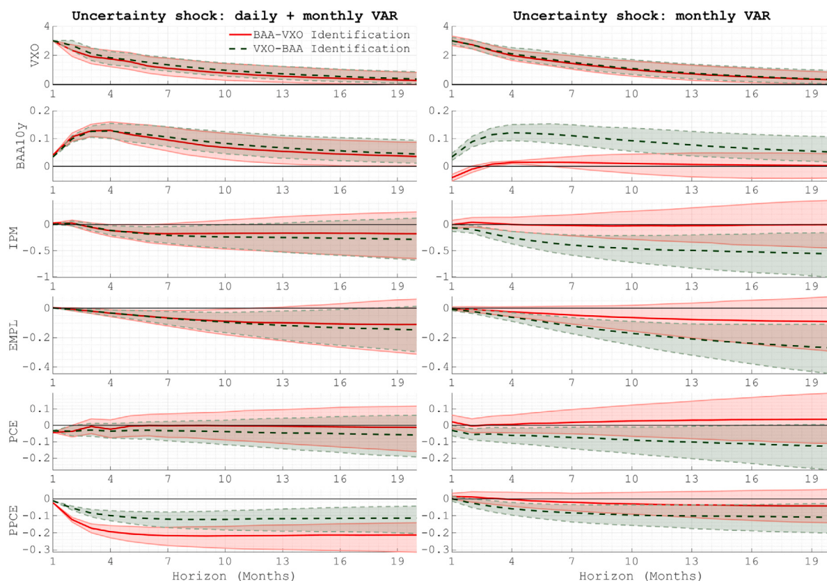
Fig. 4. Daily versus monthly identification in CFGZ.
