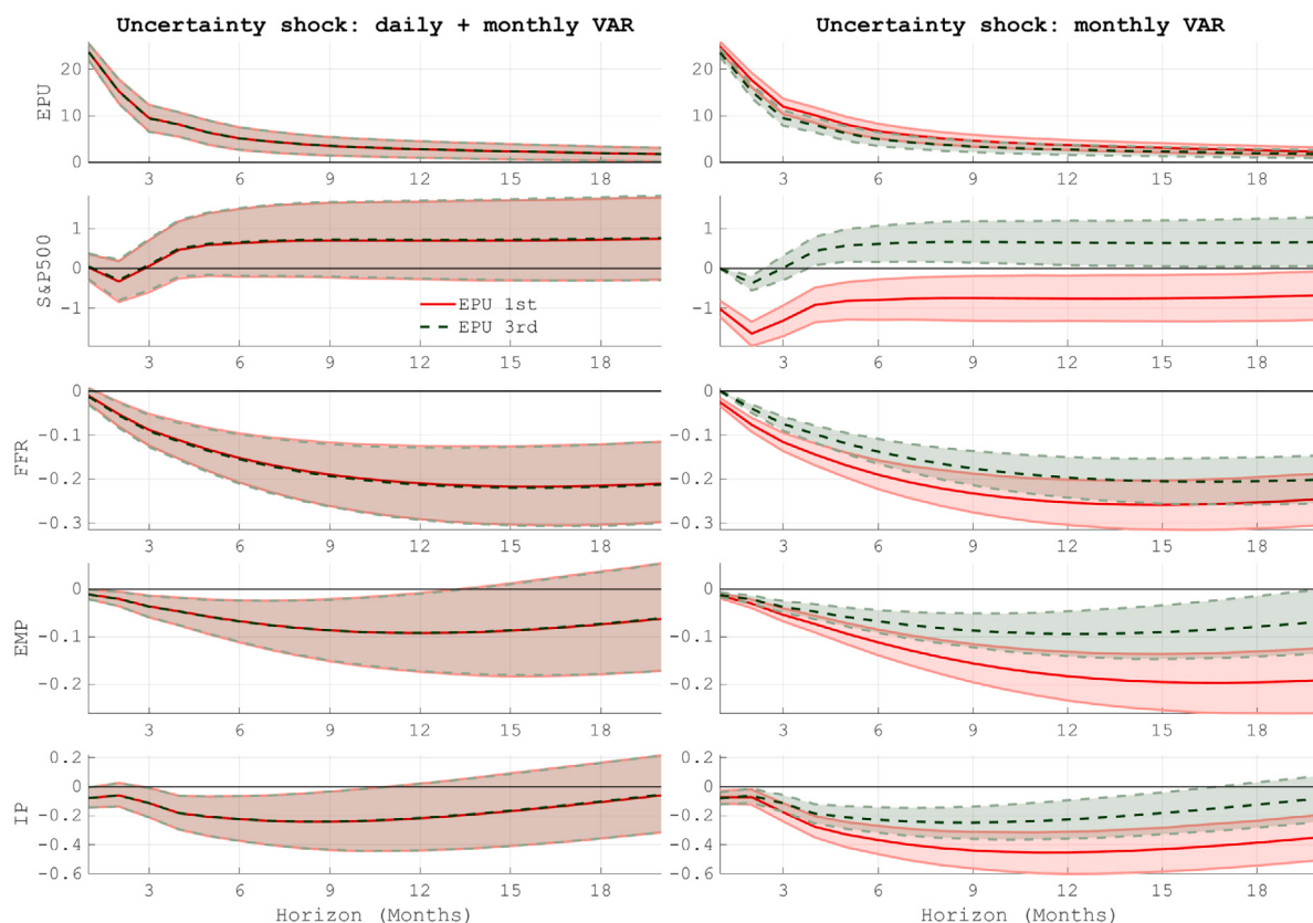
Fig. 5. Daily versus monthly identification in BBD.
