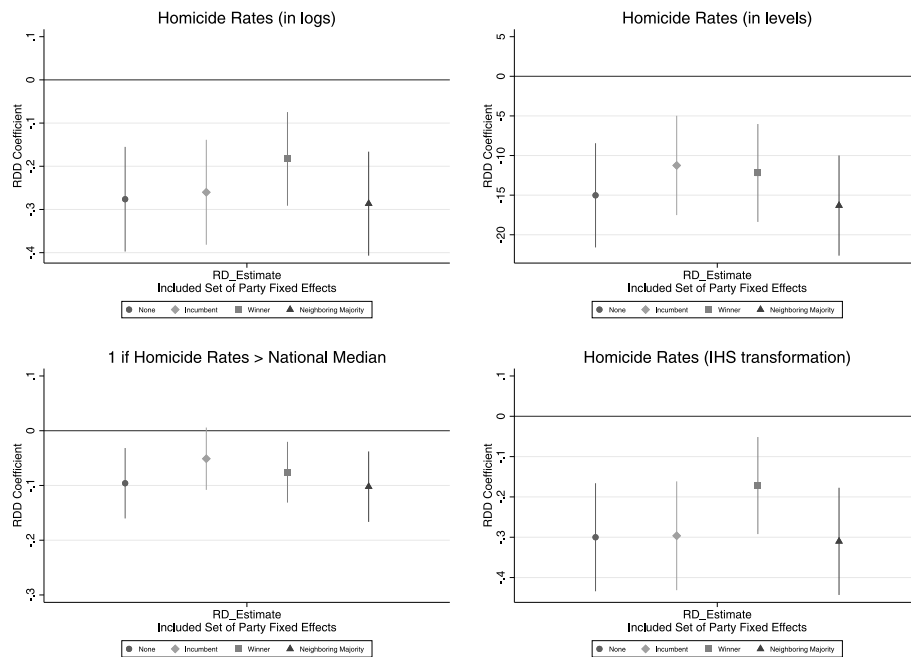
Fig. A.13. Robustness to party fixed effects (Crime). Notes: Figures plot the RDD coefficients and the 95 % confidence intervals from separate regressions when using a different set of fixed effects in our crime analysis. Estimations use an optimal bandwidth. The sample used is the same as in Table 6.
