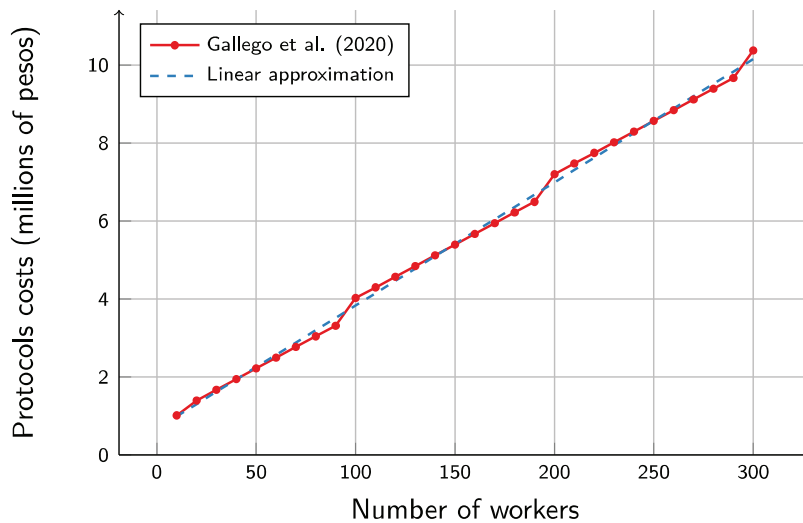
Fig. 1. Protocols costs.
