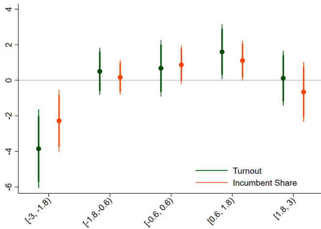
Fig. 6. Main effects for the interaction of average treatment with news, by bins of news
