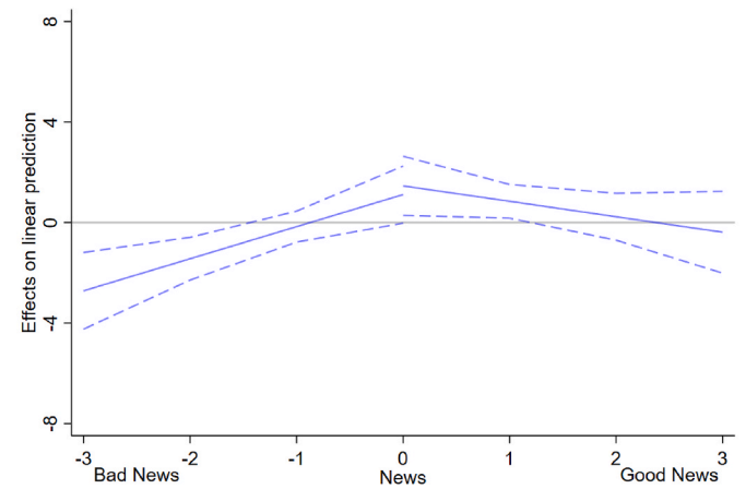
Fig. 7. Marginal effect of average treatment depending on news
