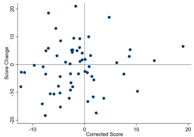
Fig. 3. Correlations between Corrected Scores and Changes in Scores for the mayoral term.
