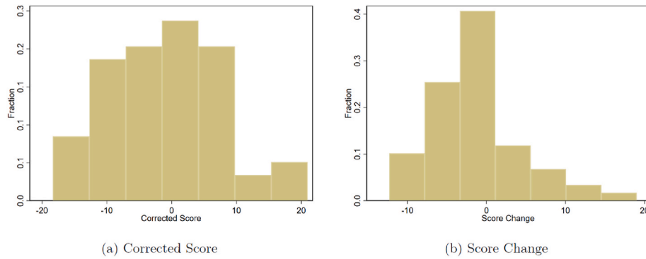
Fig. 1. Distribution of main educational outcomes
