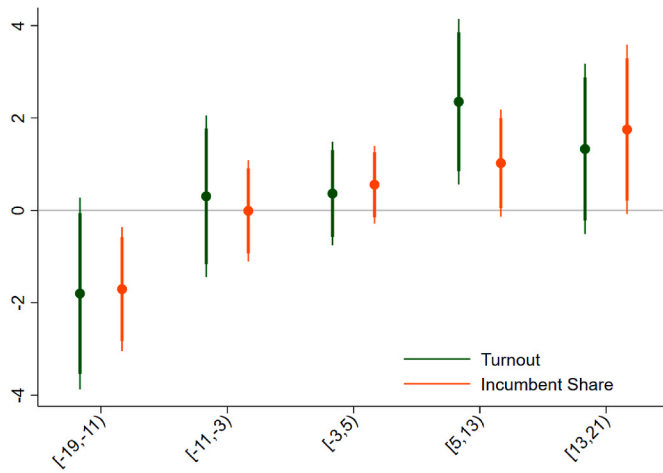
Fig. 4. Main effects for the interaction of average treatment with score, by bins of score
