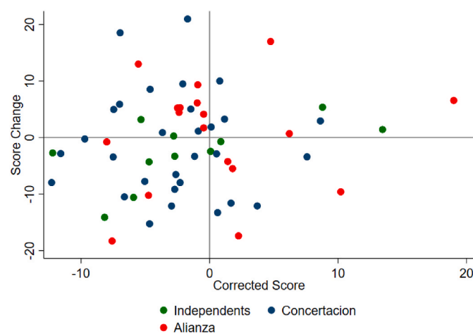
Fig. A4. Correlation between SIMCE Corrected Scores and Changes in Scores, by political coalition
