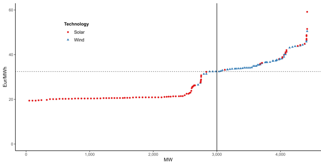
Fig. 1. The Expected Aggregate Supply Curve for Solar and Wind Investment Projects in Spain, 2019.
