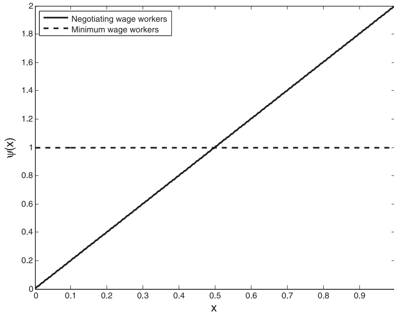
Fig. 6. Comparing the \tilde{\psi}(x) and \bar{\psi}(x) densities, example with \beta = 1/2 and \chi = 1 .
