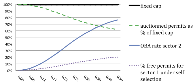
Fig. 1. Optimal policy as a function of uncertainty ( \lambda ).
