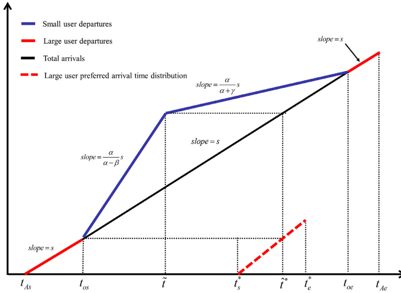
Fig. 3. PSNE in which large user does not queue (Case 1).
