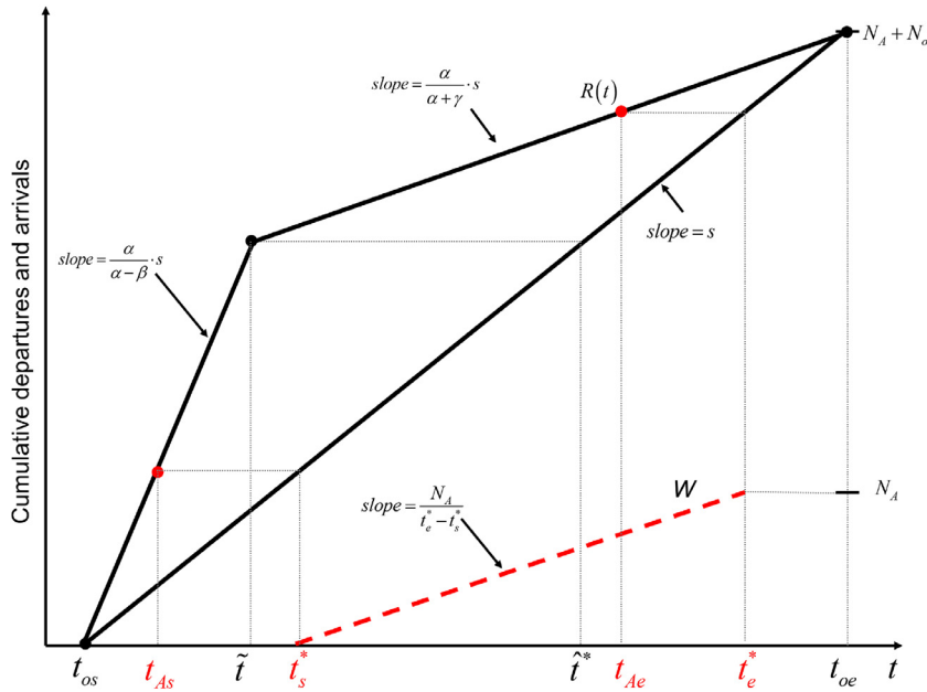
Fig. 4. PSNE in which large user does not queue (Case 2).
