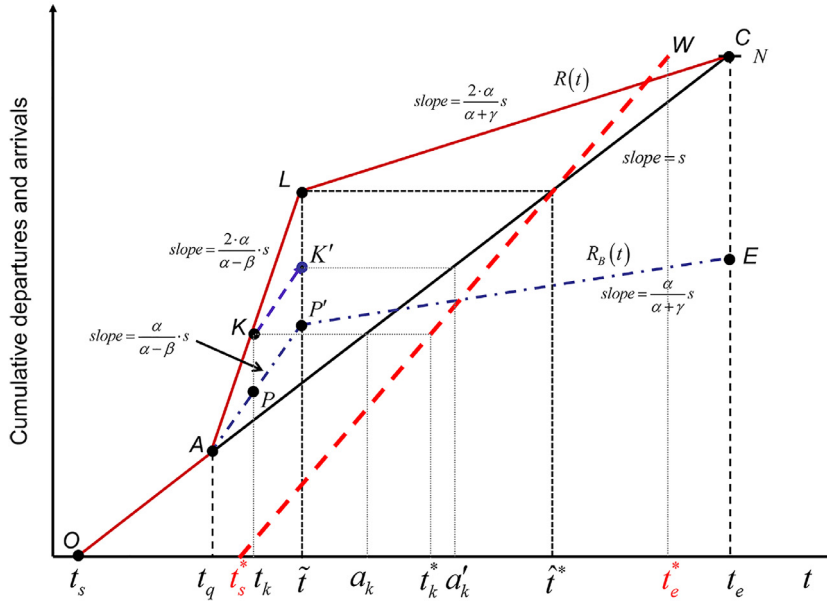
Fig. 2. PSNE with two large users.
