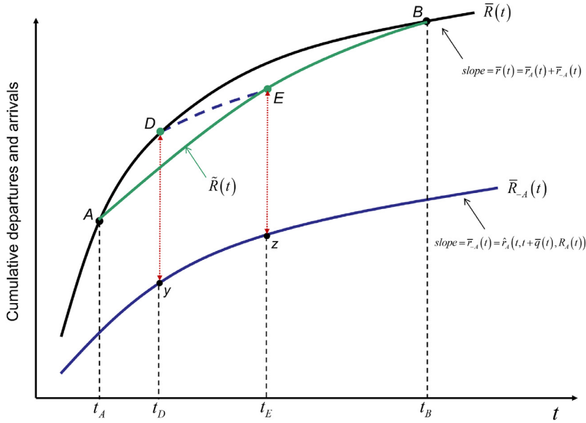
Fig. 1. Candidate PSNE with C_{aa}^A > 0 .
