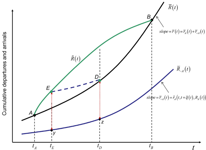
Fig. B.5. Candidate PSNE with C_{aa}^A < 0 .
