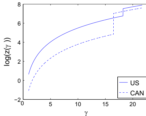
Fig. 5. Innovation before tariff drops. Graph shows the log of innovation levels ( \log(z(\gamma)) ) for different firm types ( \gamma ) in the United States (solid line) and Canada (dashed line) before the tariff reduction in the Free Trade Agreement. Innovation levels are the outcome of the equilibrium in the model.
