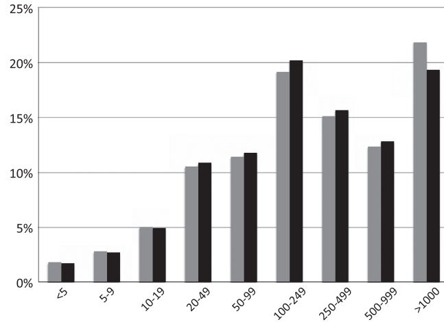
Fig. 2. Comparison of the 1992 and 1997 firm size distributions in the United States. The grey bars show the firm size distribution by employees in the manufacturing sector in the United States in 1992, and the black bars are for 1997. The vertical axis shows the percentage of employees in firms of size x . The horizontal axis shows the size of the different firms in terms of employees. Source: Bureau of Labor Statistics.
