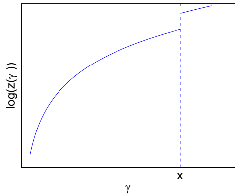
Fig. 4. Innovation as a function of firm type ( z(\gamma) ). The figure shows that innovation is an increasing function of firm type. It is continuous except when firms switch from being non-exporters ( \gamma \leq x ), to exporters ( \gamma > x ). At the export threshold, the function makes a discontinuous jump.
