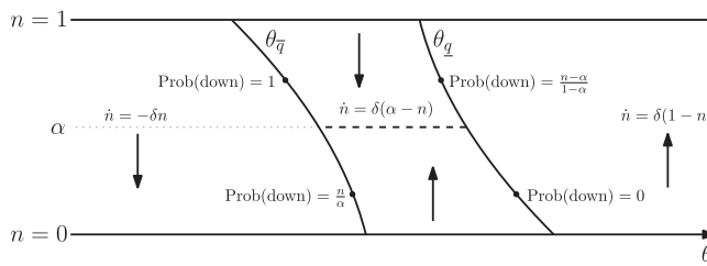
FIGURE 17 Bifurcation probabilities with two thresholds
