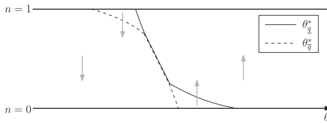
FIGURE 19 Equilibrium with small heterogeneity and \sigma \rightarrow 0
