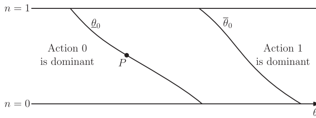
FIGURE 3 Dominance regions
