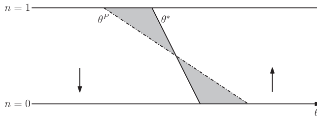
FIGURE 11 Planner's solution with linear utilities
