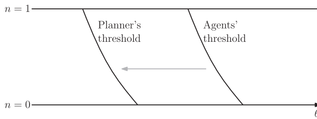
FIGURE 14 Planner's translation
